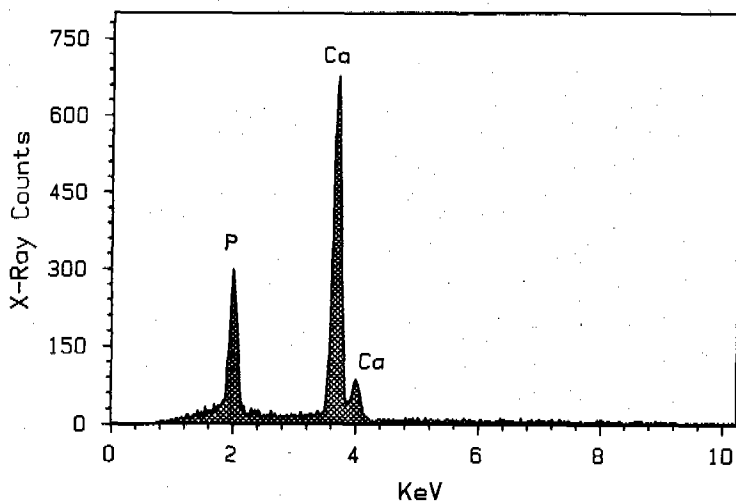
FIG. 8—EDXA spectrum typical of all five of the particles removed from Bullets 2 and 3. Note the peaks at 3.76 and 4.02 keV corresponding to the K-alpha and K-beta transitions of calcium, and the peak at 2.02 keV which represents the K-alpha transition of phosphorus. Spectra obtained from known specimens of bone demonstrated the same elements in essentially identical proportions.
