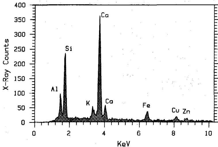
FIG. 6—This spectrum was obtained from one of the many samples of limestone rock. Note the major peaks corresponding to calcium as well as the lesser peaks of aluminum and silicon. Trace quantities of other elements are present.
