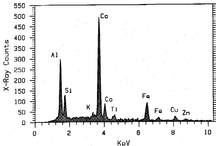
FIG. 5—This EDXA spectrum of particle B again demonstrates major peaks at 3.76 and 4.02 keV typical of calcium, as well as the smaller peaks of aluminum and silicon, and the copper and zinc peaks. There are also trace quantities of iron (6.40 keV) and titanium (4.51 keV) within this fragment of mineral. These last elements not only occur as "impurities" in a variety of minerals, but they are common elements in pigments used by masons or painters.
